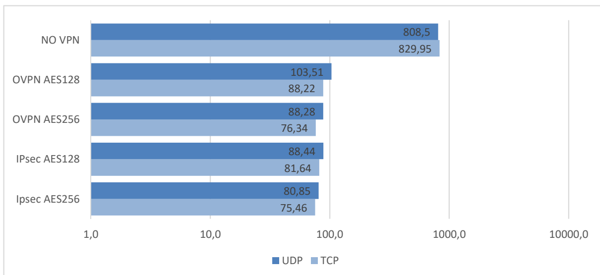
Performance COMPACT SMALL UTM (N2930) [Mbps]
