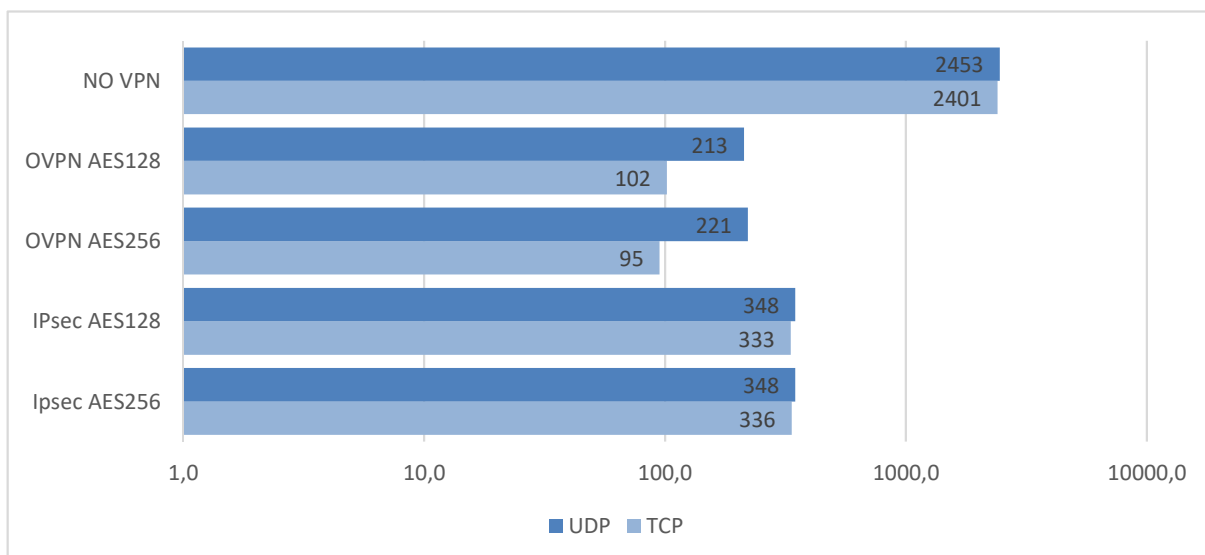
Performance COMPACT SMALL UTM 4 (J6412) [Mbps]
