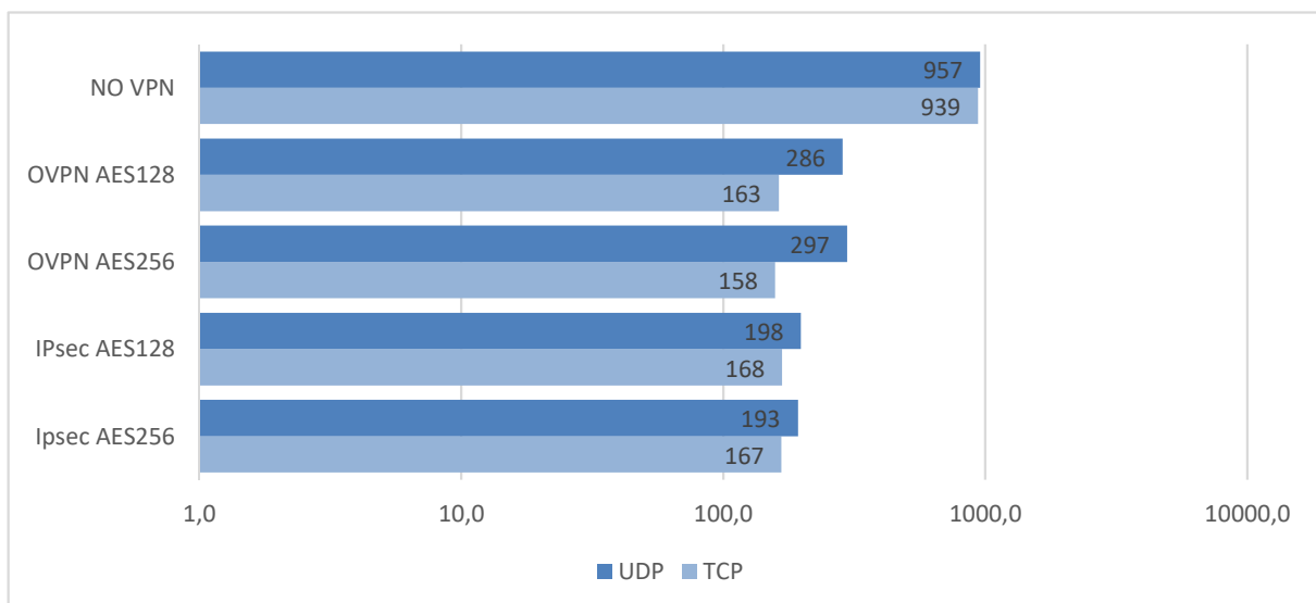
Performance Appliance B1 8 core (C3758) [Mbps]
